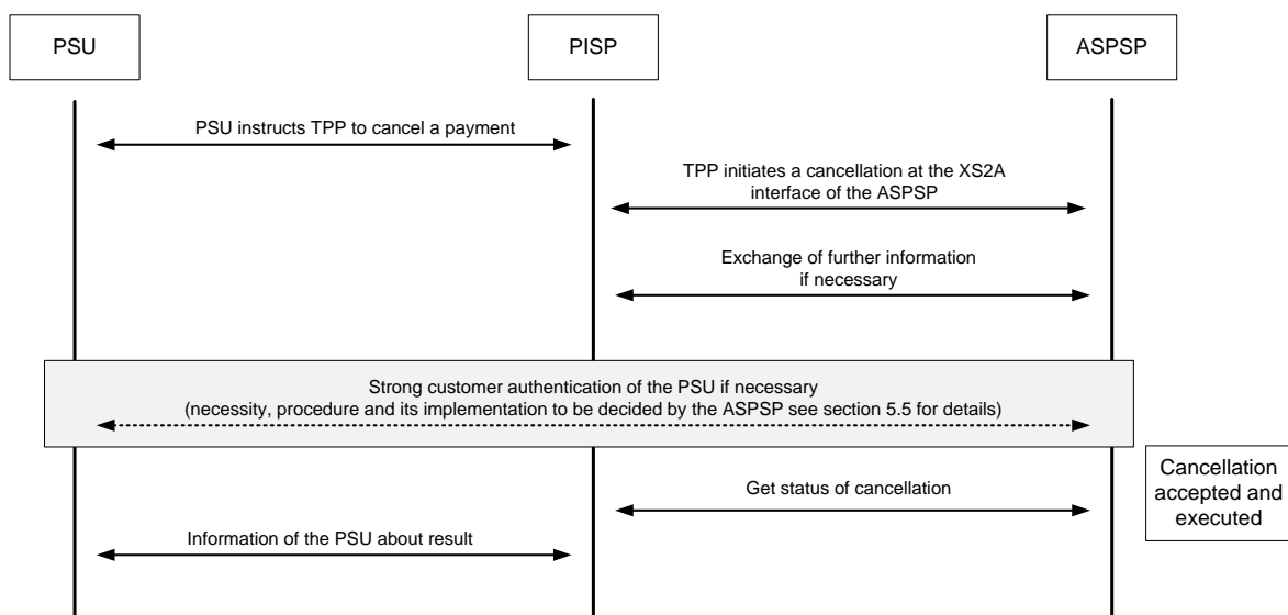
Figure 7: Use case Cancellation of a payment
