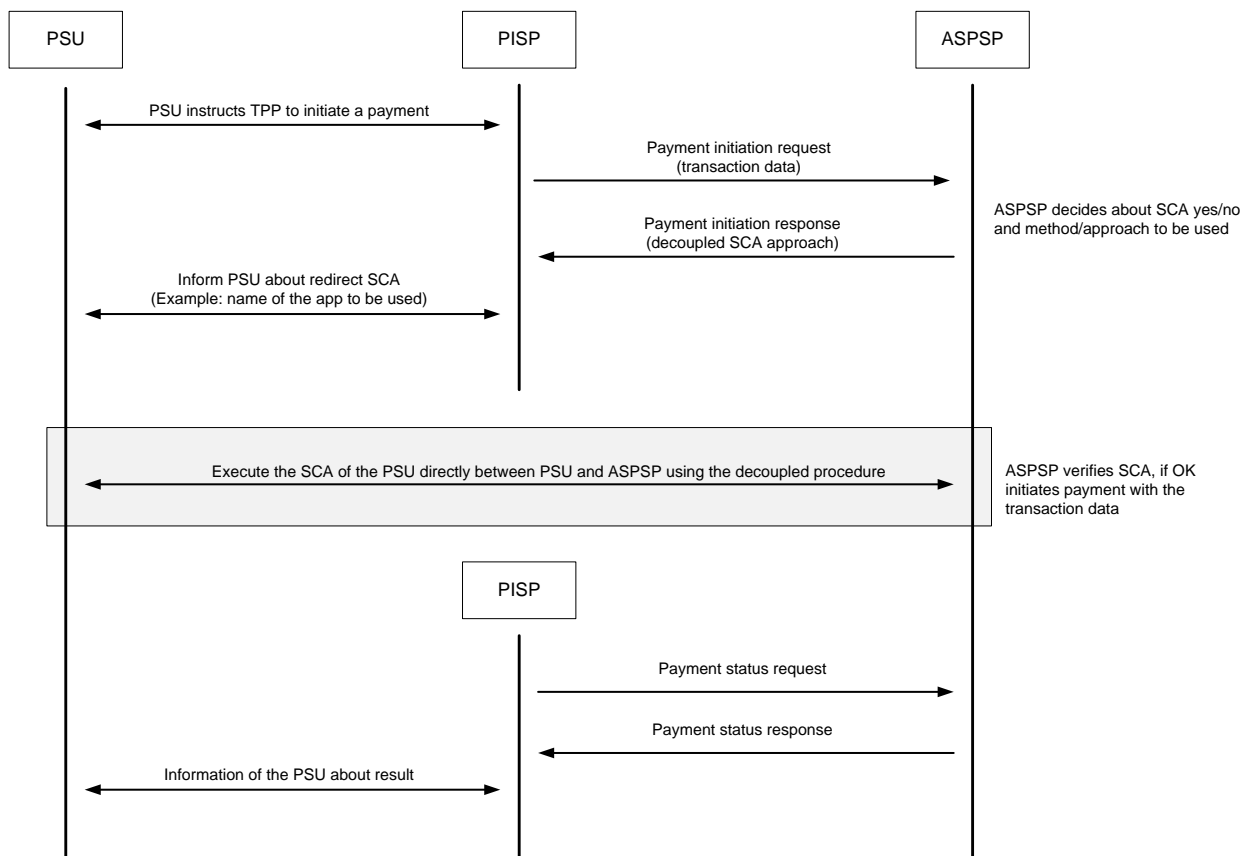
Figure 19: Decoupled approach for SCA
